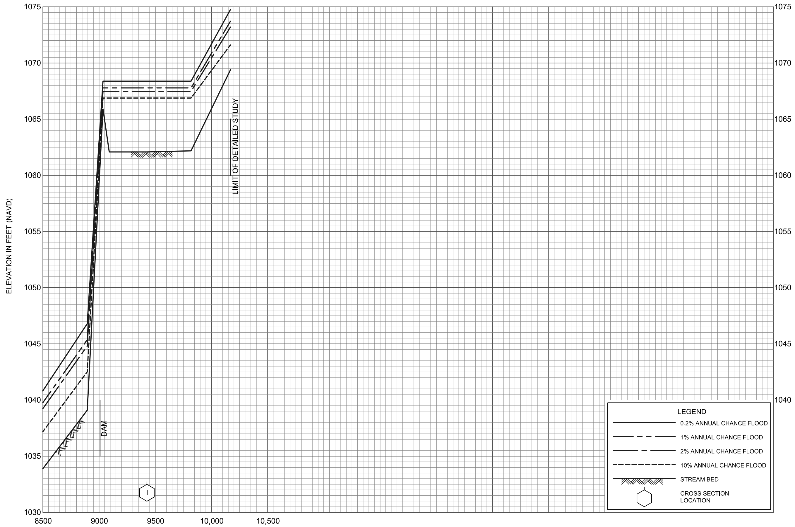
STREAM DISTANCE IN FEET ABOVE CONFLUENCE WITH BEAVER CREEK
